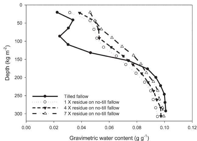
Fig. 3. Average seed-zone water content over the 6-yr period (each point is the mean of 6 yr and four replications). Treatments are significantly different at 200 kg m -2 ( p > F = 0.0016 ). All non-adjacent means at 200 kg m -2 are significantly different at p > |t| = 0.04 . The year by treatment interaction was not significant.
