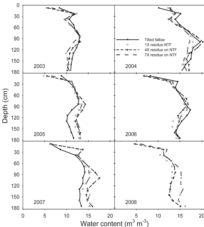
Fig. 4. Volumetric water content at the end of the fallow period to a depth of 180 cm from 2003 to 2008. Each data point is the mean of four replications. NTF = no-till fallow.
