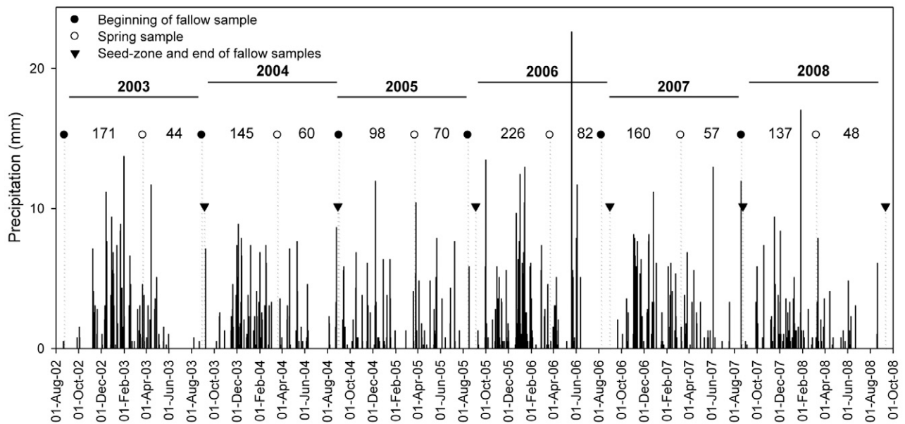
Fig. 1. Daily precipitation during the 2003 to 2008 fallow periods at Lind, WA. Also shown is the timing of 180-cm deep volumetric water profile measurements obtained each year at the beginning of the fallow period, in the spring of the fallow period, and at the end of the fallow period. Total precipitation (mm) between those points is noted. The date when incremental seed-zone water samples were obtained is indicated by a triangle. Horizontal bars indicate individual fallow periods and are labeled with the year the fallow period ends.
